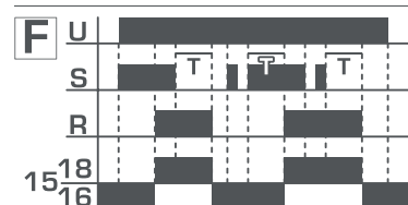
Signal ON and OFF delay
